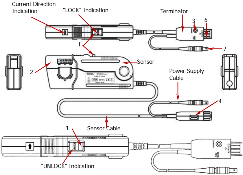
Figure 2 RP1005C Parts
