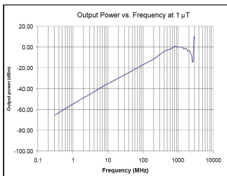
12mm magnetic field sniffer
